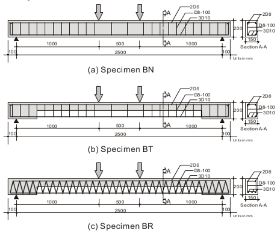
Fig. 2 Detail of Specimens
