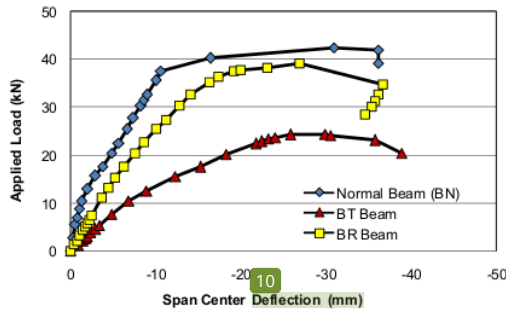
Fig. 7 Typical Load-Deflection Relationship
