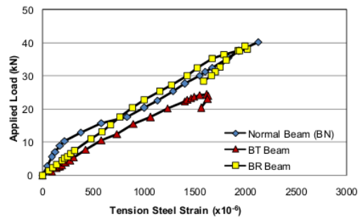
Fig. 8 Strain of the tensile reinforcement
