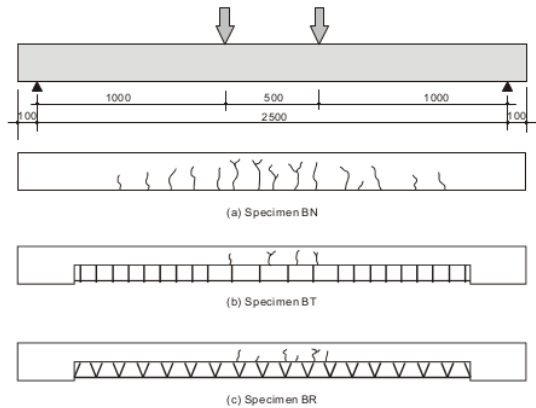
Fig. 11 Typical Crack Pattern of Specimens
