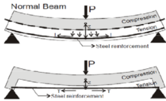
Fig. 5 Illustration of Flexural Action of Specimen BT
